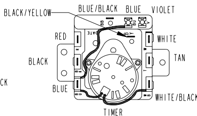
WIRING DIAGRAM - GAS
