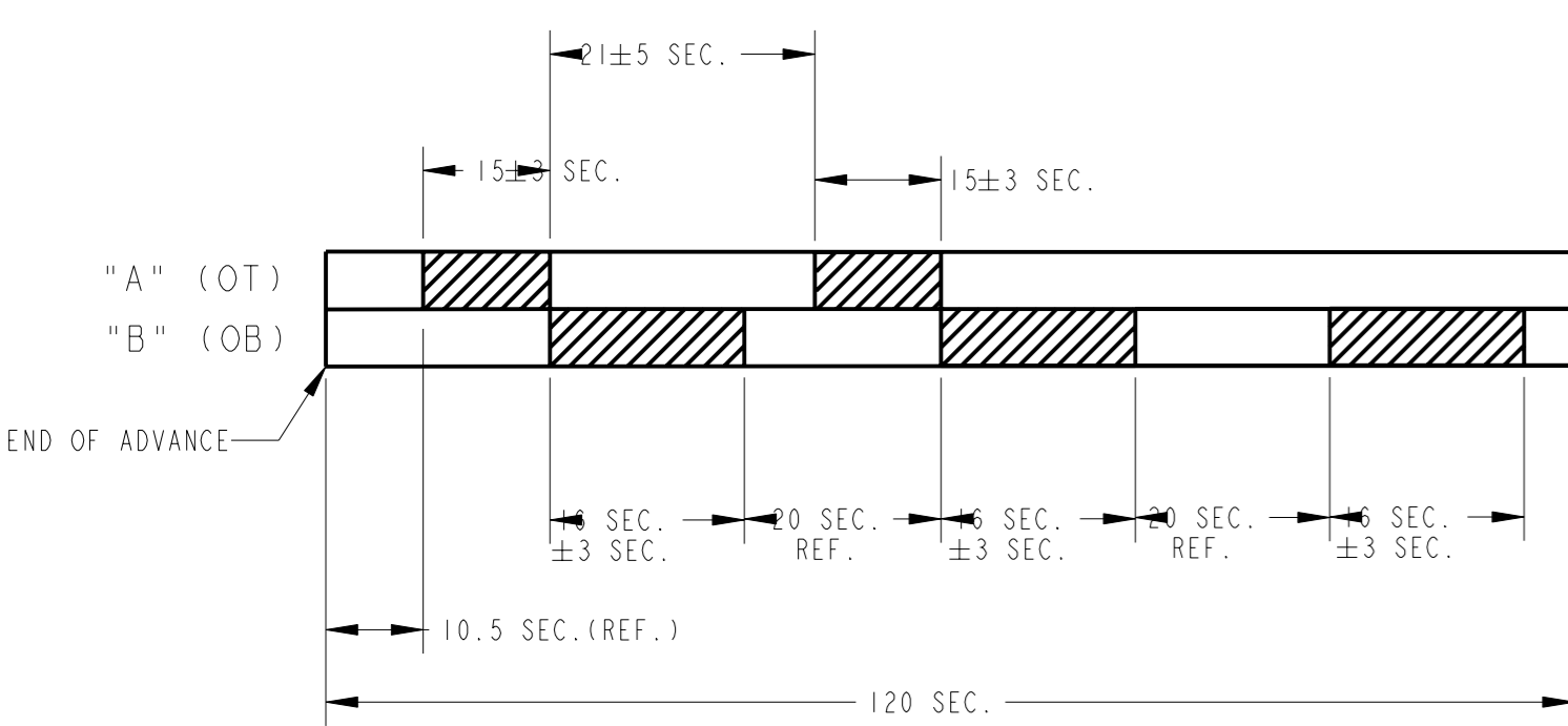
SUBINTERVAL TIMING
