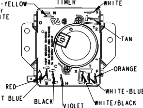
WIRING DIAGRAM - GAS
