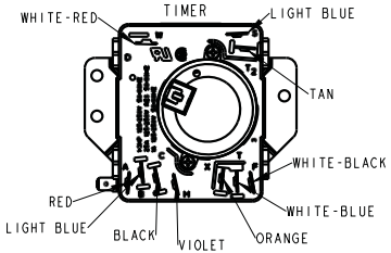
WIRING DIAGRAM - GAS
