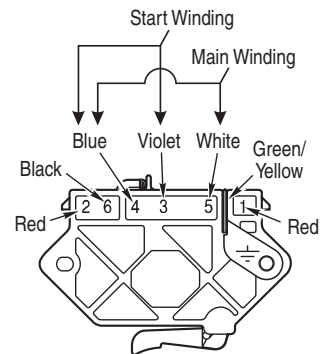
Pluggable Drive Motor Switch
