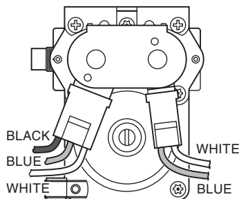
Gas Valve
