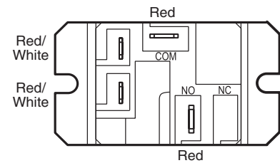
Heater Relay
