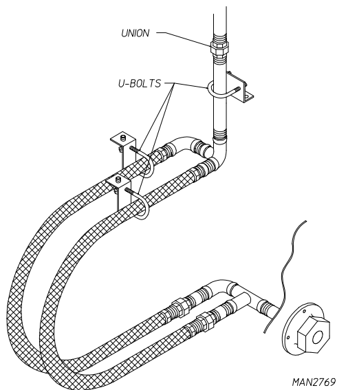
GAS FLEX HOSE UNION RECONNECTION VIEW ②
