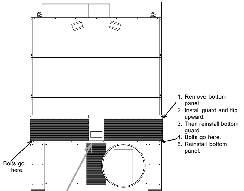
REAR VIEW
