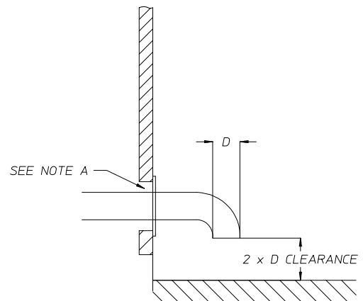
HORIZONTAL DUCTING
