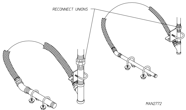
STEAM FLEX HOSE UNION RECONNECTION VIEW ②
