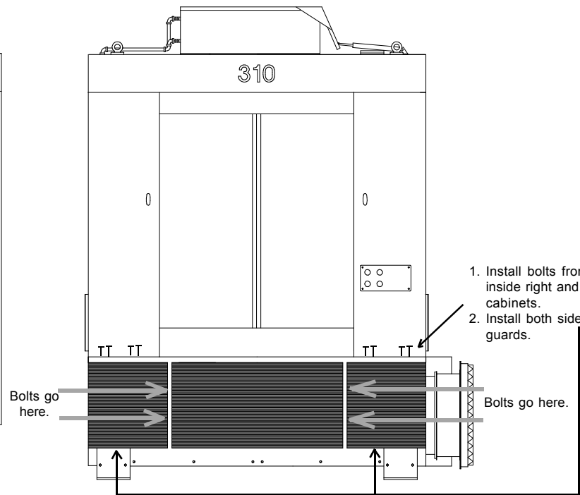
REAR VIEW
