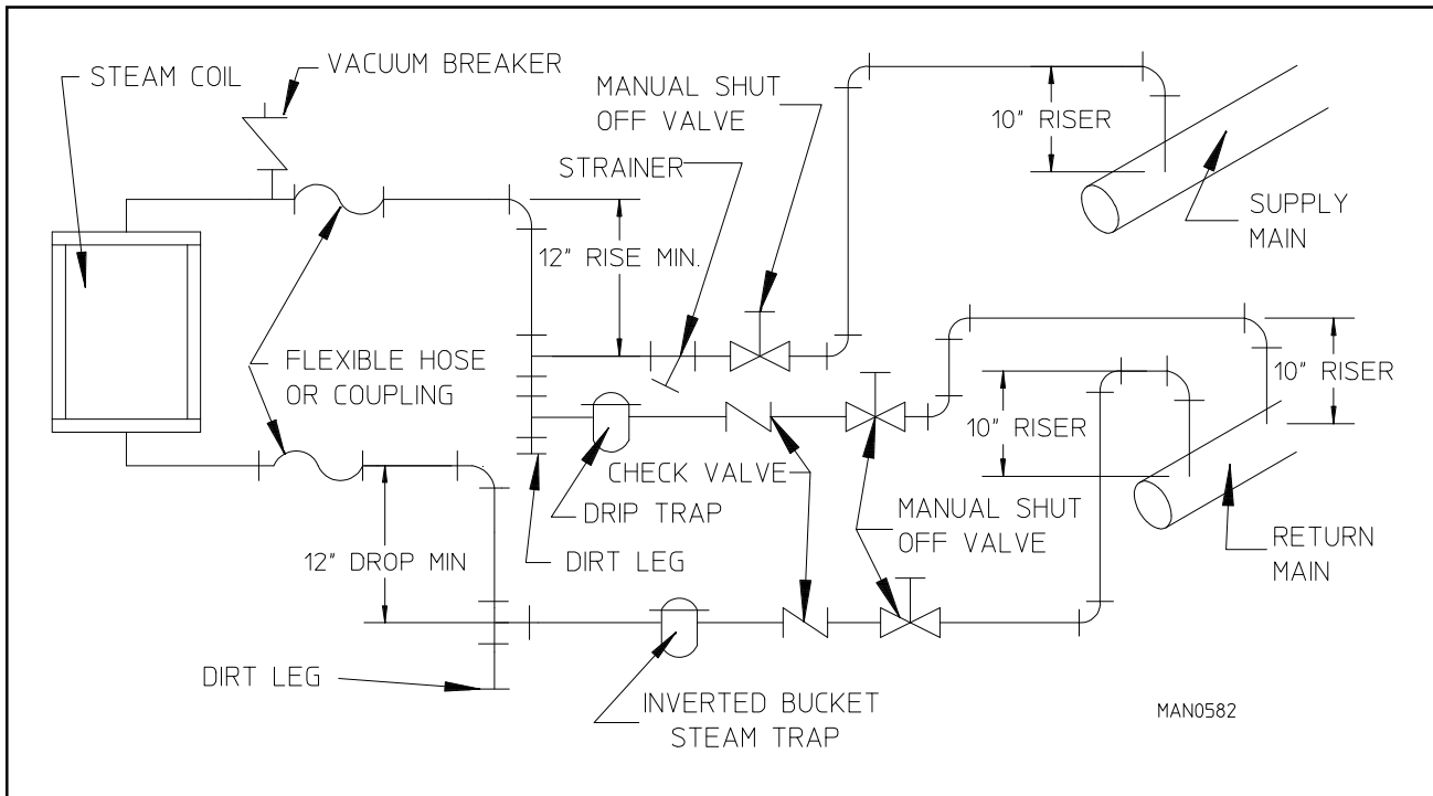
STEAMDAMPER SYSTEM
