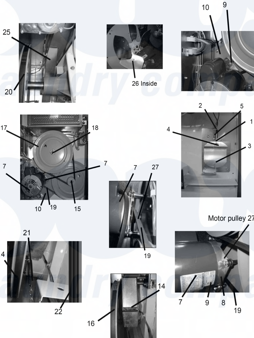
Dexter Commercial Dexter DDAD30 Dryer Parts Parts Diagram Rear View Click on the part number to view part
