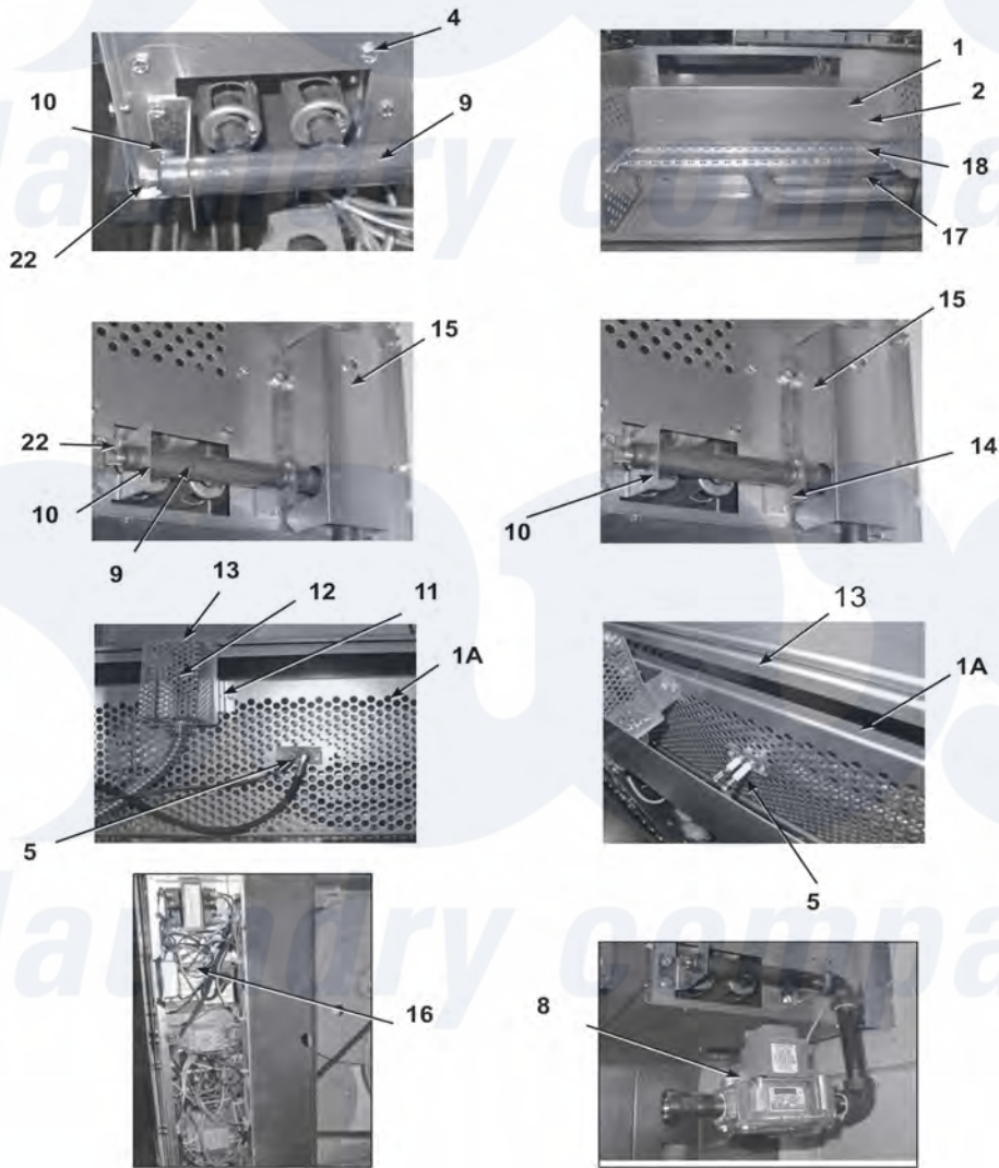
Dexter Commercial Dexter DDAD50KC Dryer Parts Parts Diagram Burner Housing Group
