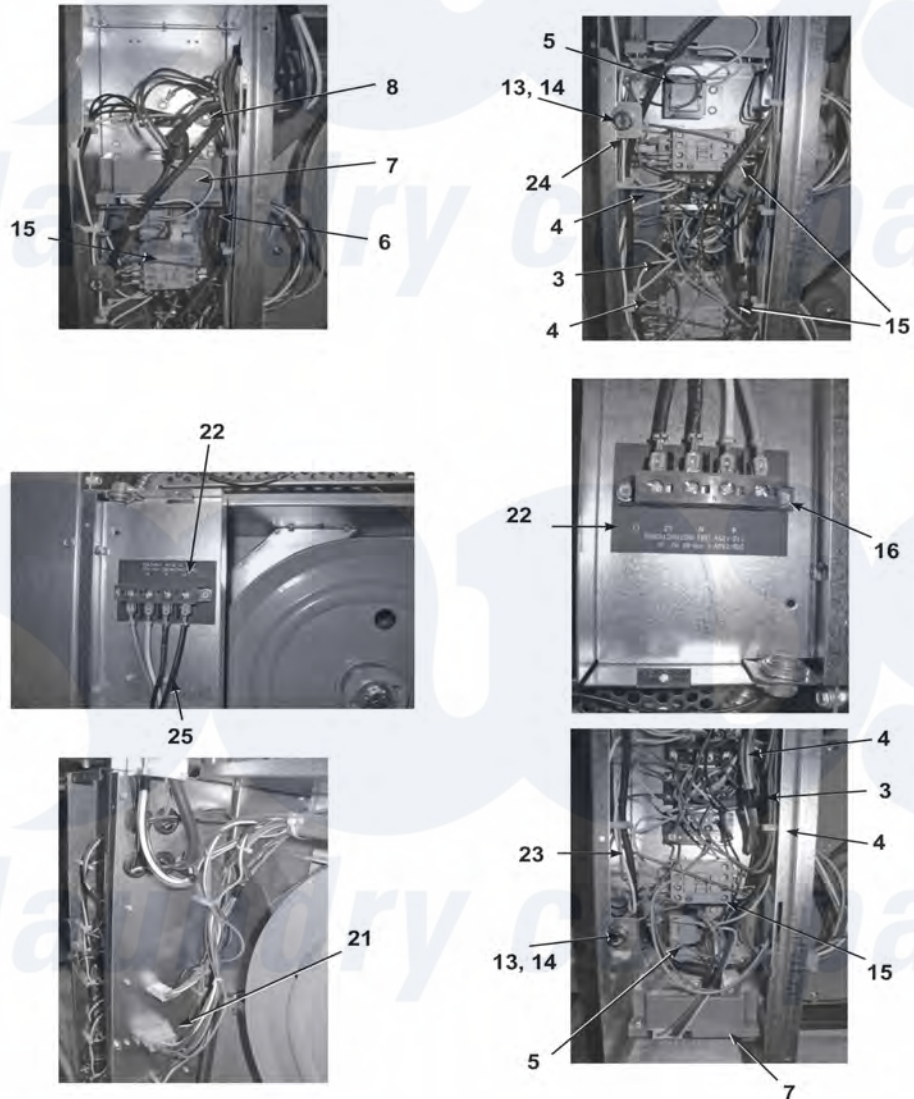
Dexter Commercial Dexter DDAD50KC Dryer Parts Parts Diagram Control Assembly Group Click on the part number to view part
