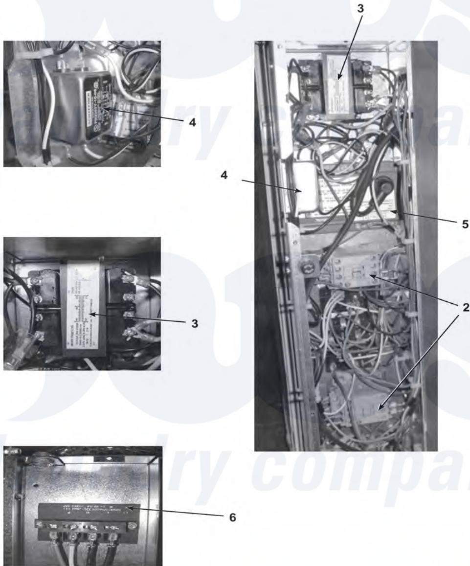
Dexter Commercial Dexter DDAD50KC Dryer Parts Parts Diagram Electrical Group Click on the part number to view part
