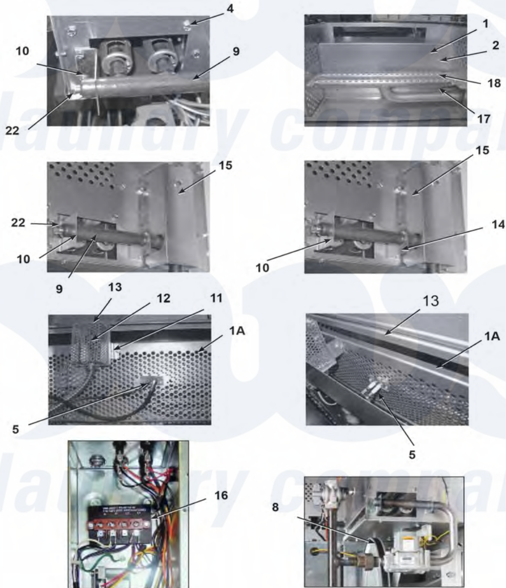
Dexter Commercial Dexter DDBD50 (Spring 2011) Dryer Parts Parts Diagram Burner Housing Group Click on the part number to view part
