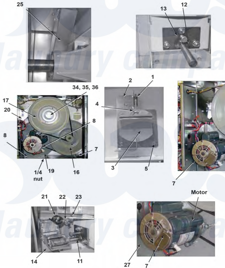
Dexter Commercial Dexter DDBD50 (Spring 2011) Dryer Parts Parts Diagram Rear View Click on the part number to view part
