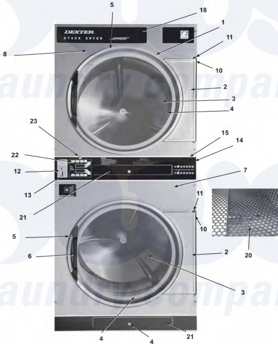
Dexter Commercial Dexter DDBD50KC Dryer Parts Parts Diagram Cabinet Group
