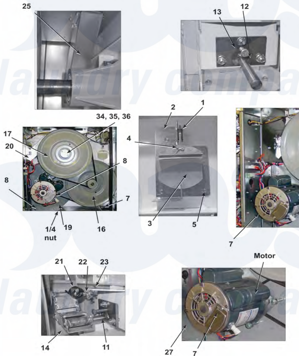
Dexter Commercial Dexter DDBD50KC Dryer Parts Parts Diagram Rear View
