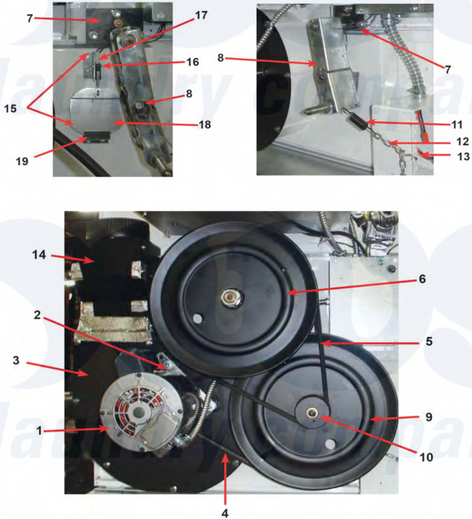
Dexter Commercial Dexter SWD Stacked Washer and Dryer Parts Parts Diagram Dryer Rear View Click on the part number to view part
