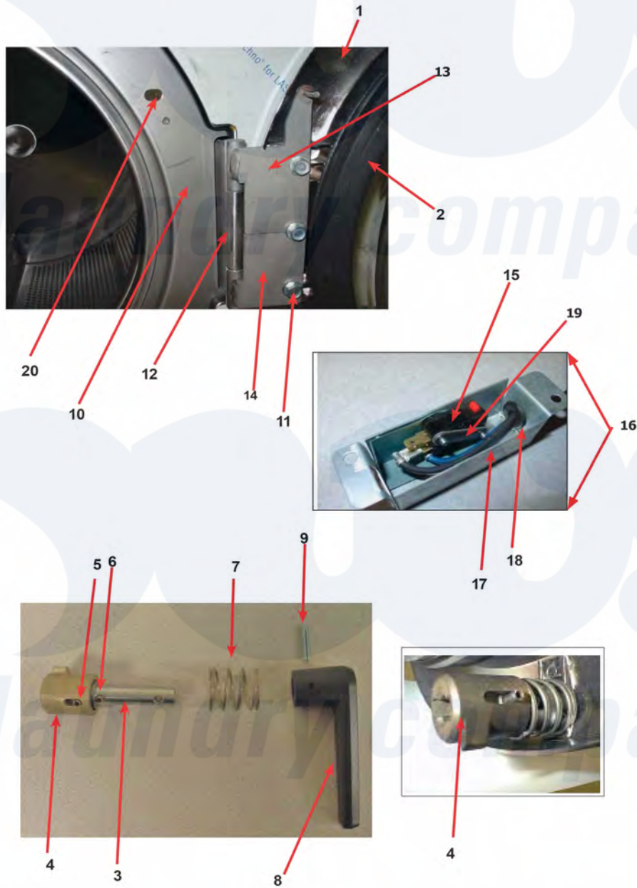
Dexter Commercial Dexter SWD Stacked Washer and Dryer Parts Parts Diagram Loading Door Hinge Click on the part number to view part
