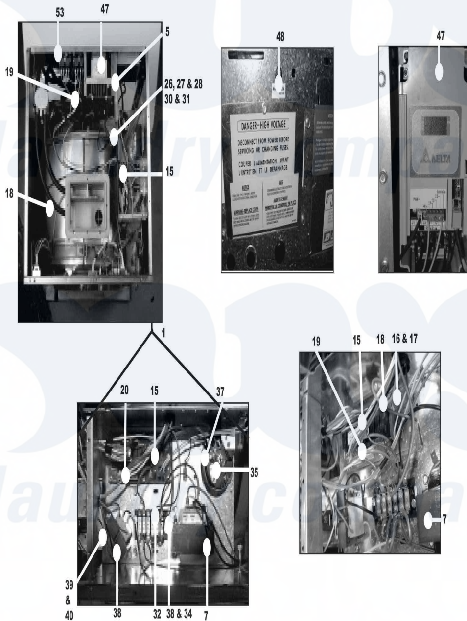
Dexter Commercial Dexter WCAD18KCS-10 (T-300) Washer Parts Parts Diagram Electrical Components Click on the part number to view part
