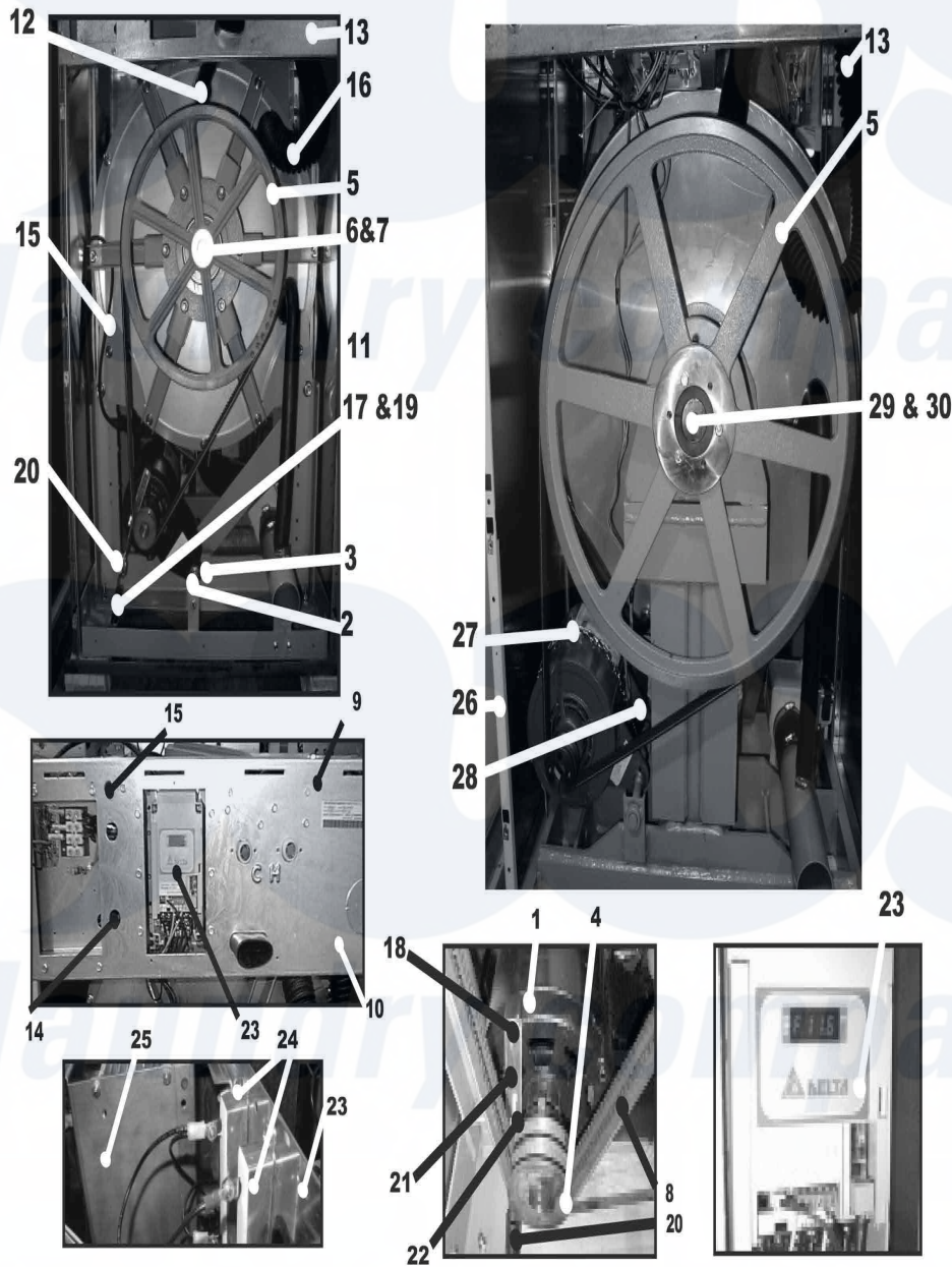
Dexter Commercial Dexter WCAD18KCS-10 (T-300) Washer Parts Parts Diagram Rear View Access Click on the part number to view part
