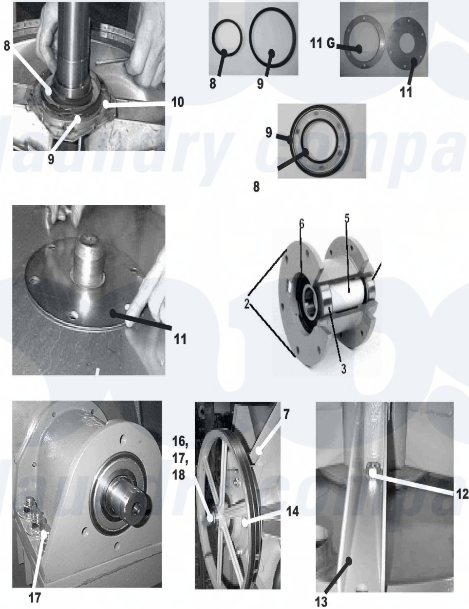
Dexter Commercial Dexter WCAD18KCS-12 (T-300) Washer Parts Parts Diagram Cylinder, Seals & Bearings Click on the part number to view part
