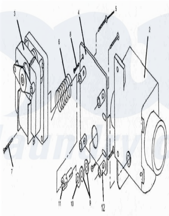
Dexter Commercial Dexter WCAD18KCS-12 (T-300) Washer Parts Parts Diagram Drain Valve Click on the part number to view part
