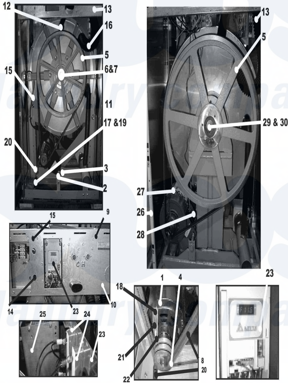
Dexter Commercial Dexter WCAD18KCS-12 (T-300) Washer Parts Parts Diagram Rear View Access Click on the part number to view part
