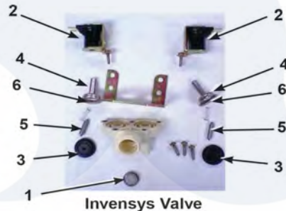
Invensys Valve
