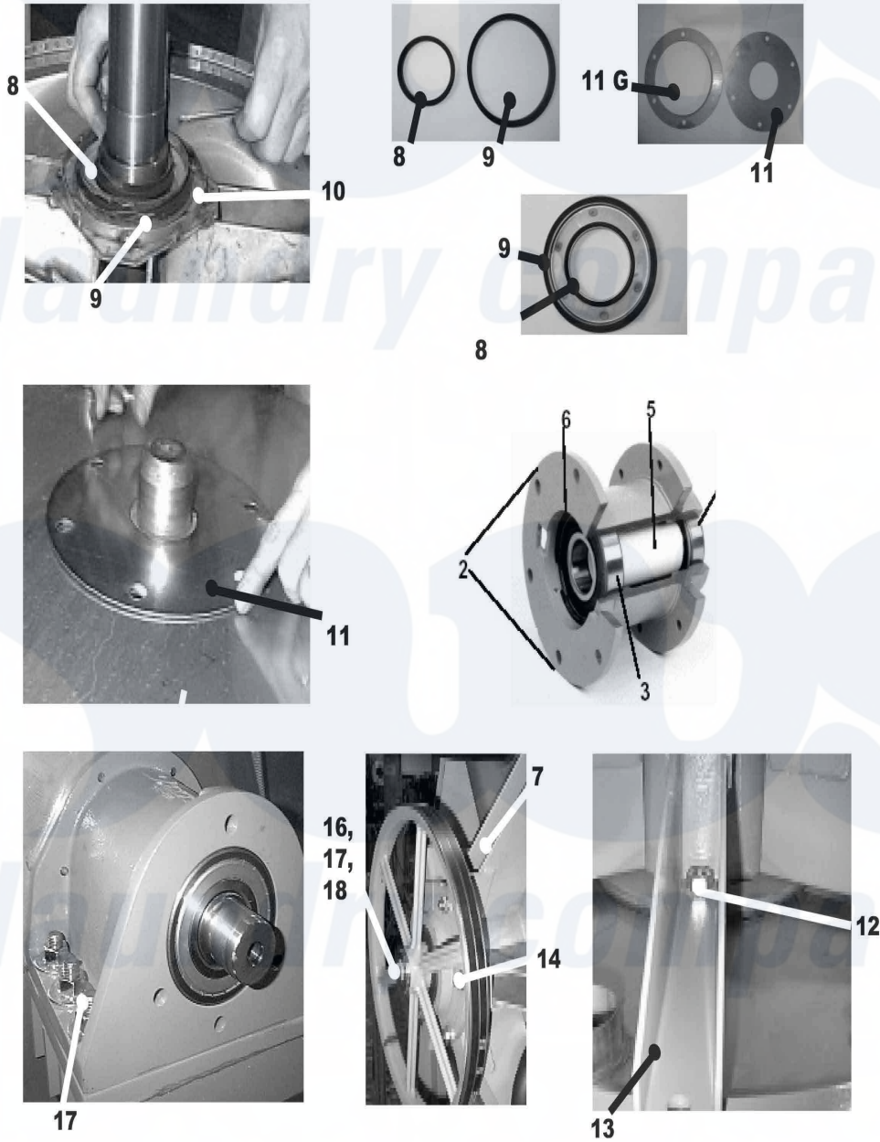
Dexter Commercial Dexter WCAD25KCS-12 (T-400) Washer Parts Parts Diagram Cylinder, Seals & Bearings Click on the part number to view part
