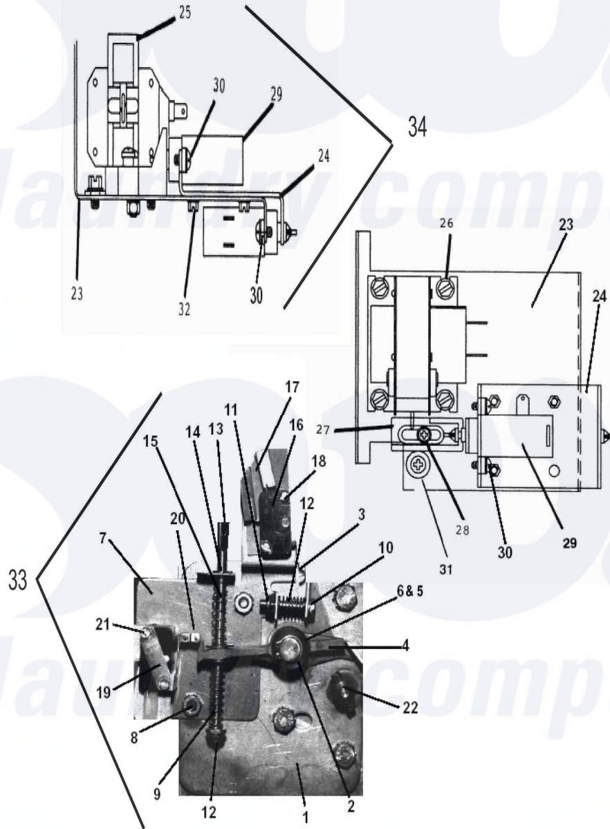
Dexter Commercial Dexter WCAD25KCS-12 (T-400) Washer Parts Parts Diagram Door Lock
