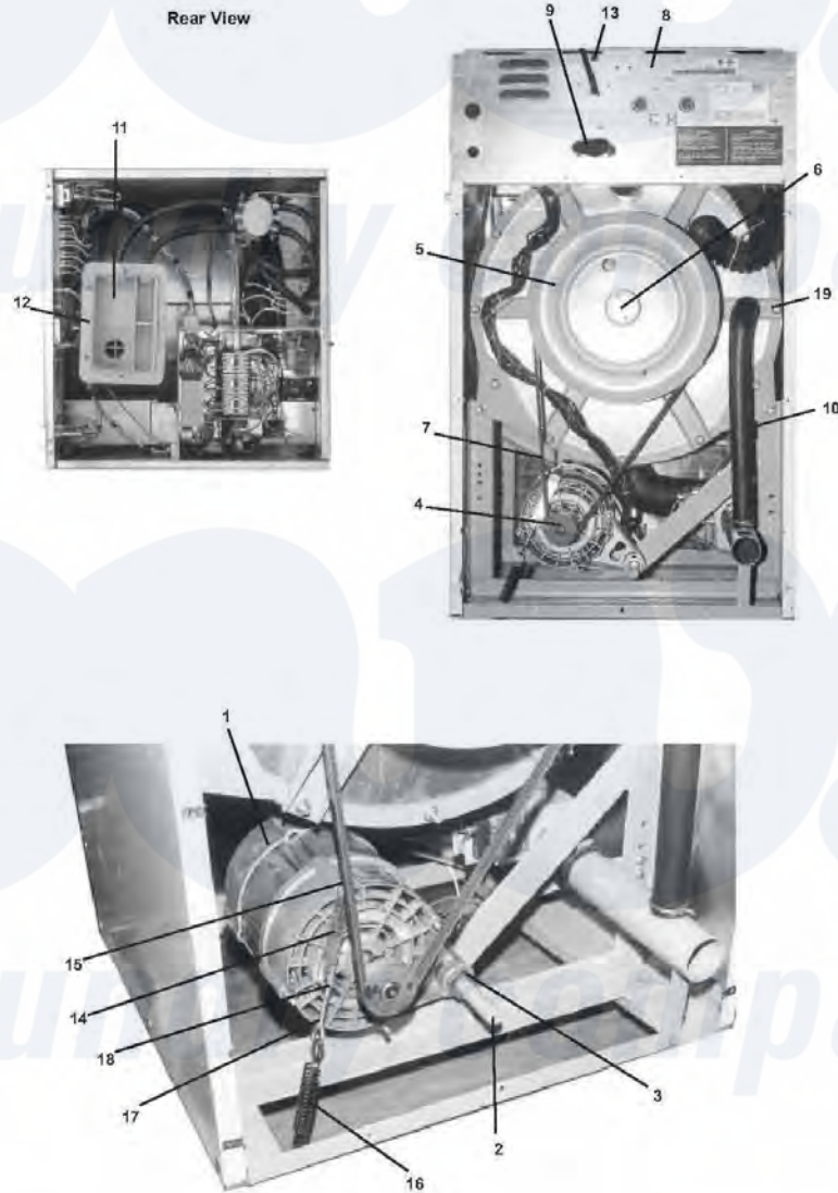
Dexter Commercial Dexter WCN18AA Washer Parts Parts Diagram Rear View Click on the part number to view part
