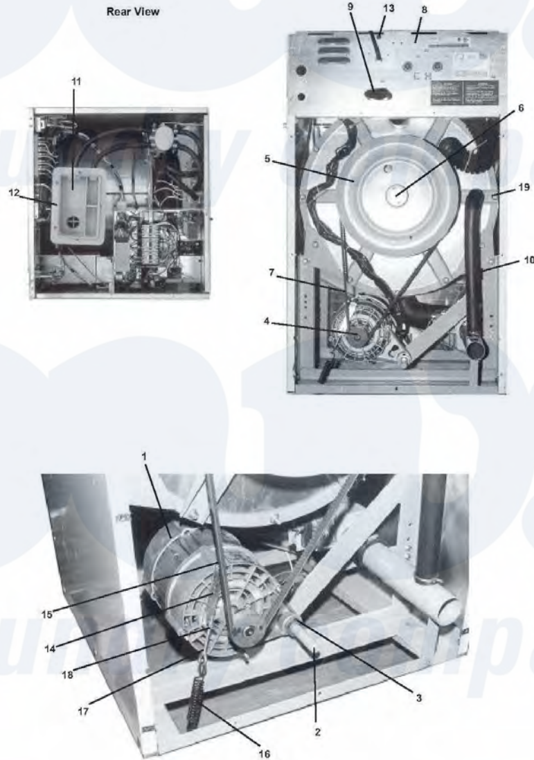
Dexter Commercial Dexter WCN18AB Washer Parts Parts Diagram Rear View Click on the part number to view part
