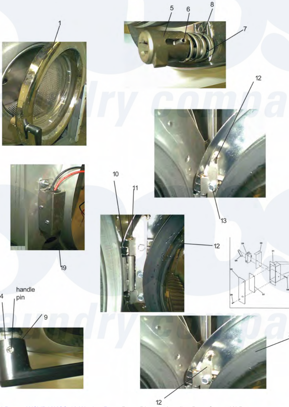
96 Dexter Commercial Dexter WCVD18KCS-10 Washer Parts Parts Diagram Loading Door Group 18LB Click on the part number to view part
