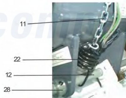
Dexter Commercial Dexter WCVD55KCS-12 Washer Parts Parts Diagram Rear View 55LB, 75LB Click on the part number to view part
