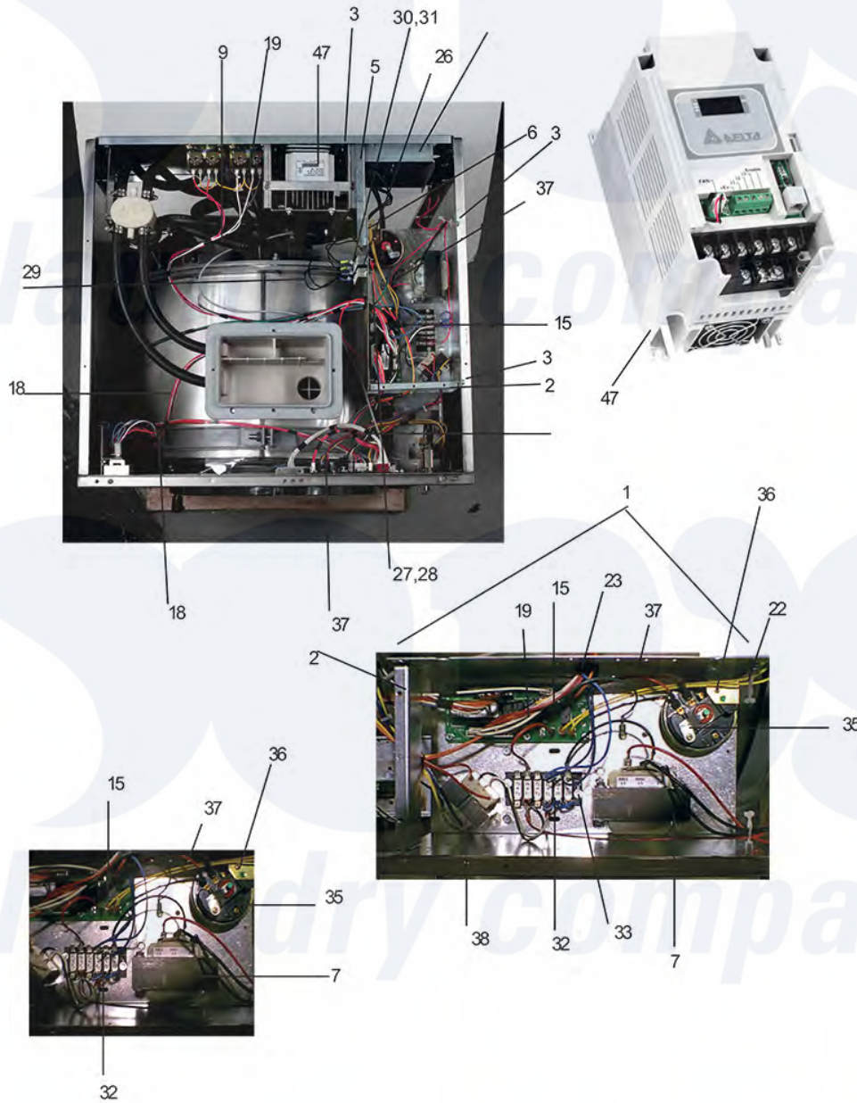
Dexter Commercial Dexter WCVD75KCS-12 Washer Parts Parts Diagram Electrical Components - Top Compartment Click on the part number to view part
