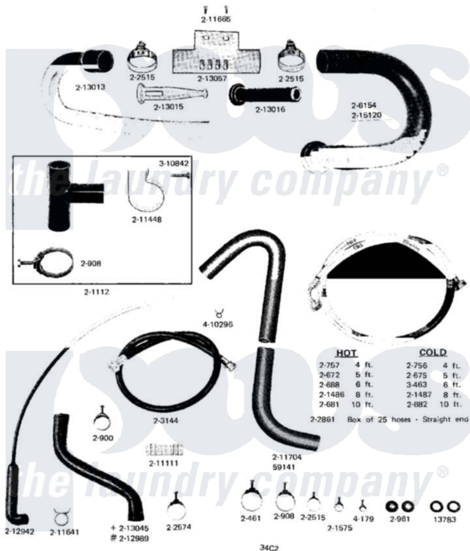
Maytag Commercial Maytag A15CM Washer Parts Parts Diagram 12 - WATER INJECTION SYSTEM, HOSES & CLAMPS
