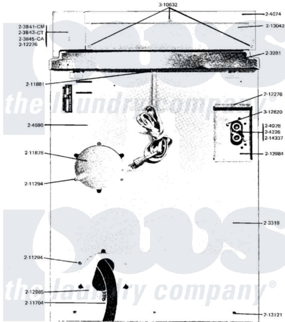
Maytag Commercial Maytag A15CT Washer Parts Parts Diagram 05 - REAR VIEW
