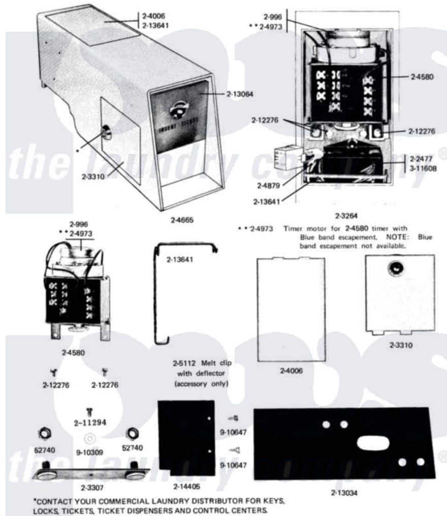
Maytag Commercial Maytag A21CT Washer Parts Parts Diagram 06 - CT CONTROL CENTER Click on the part number to view part
