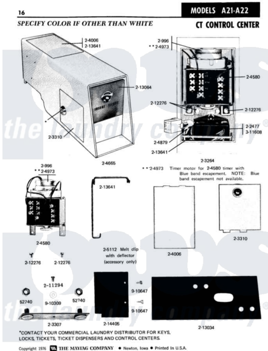
Maytag Commercial Maytag A22CT Washer Parts Parts Diagram 06 - CT CONTROL CENTER Click on the part number to view part
