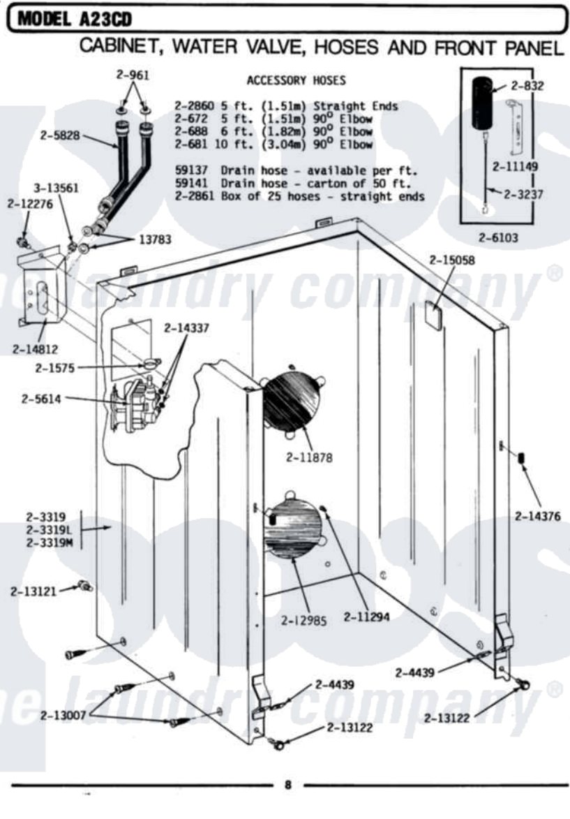
Maytag Commercial Maytag A23CDL Washer Parts Parts Diagram 04 - CABINET\WATER VALVE\HOSES\FRONT PANEL
