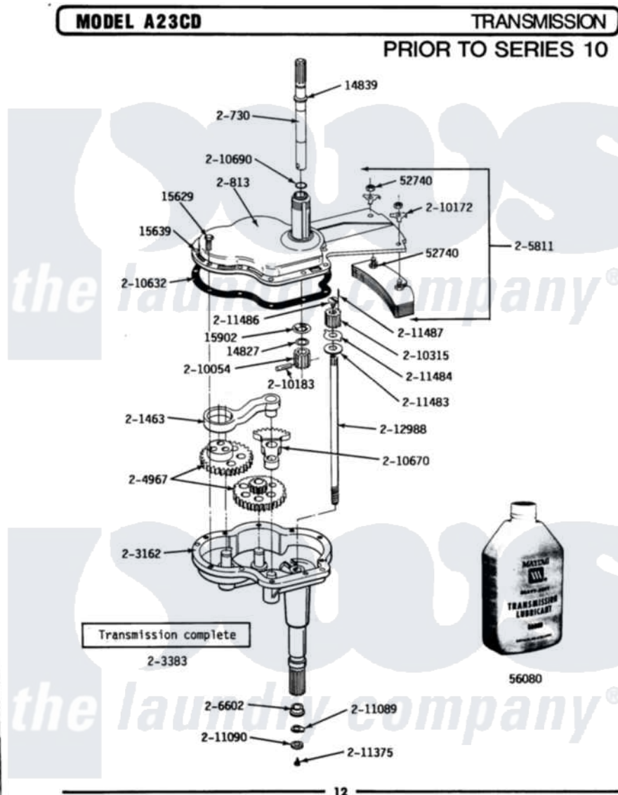
Maytag Commercial Maytag A23CDL Washer Parts Parts Diagram 06 - TRANSMISSION Click on the part number to view part
