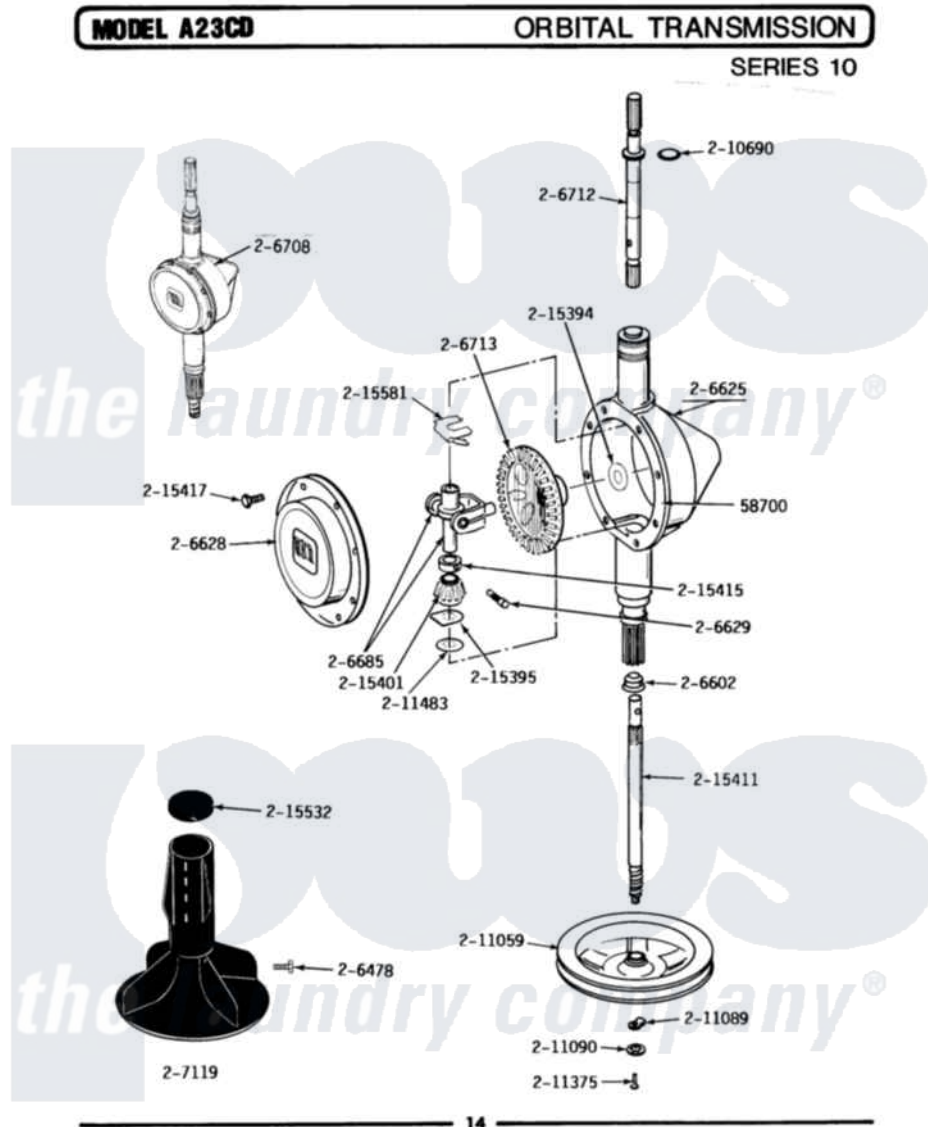
Maytag Commercial Maytag A23CDL Washer Parts Parts Diagram 07 - ORBITAL TRANSMISSION Click on the part number to view part
