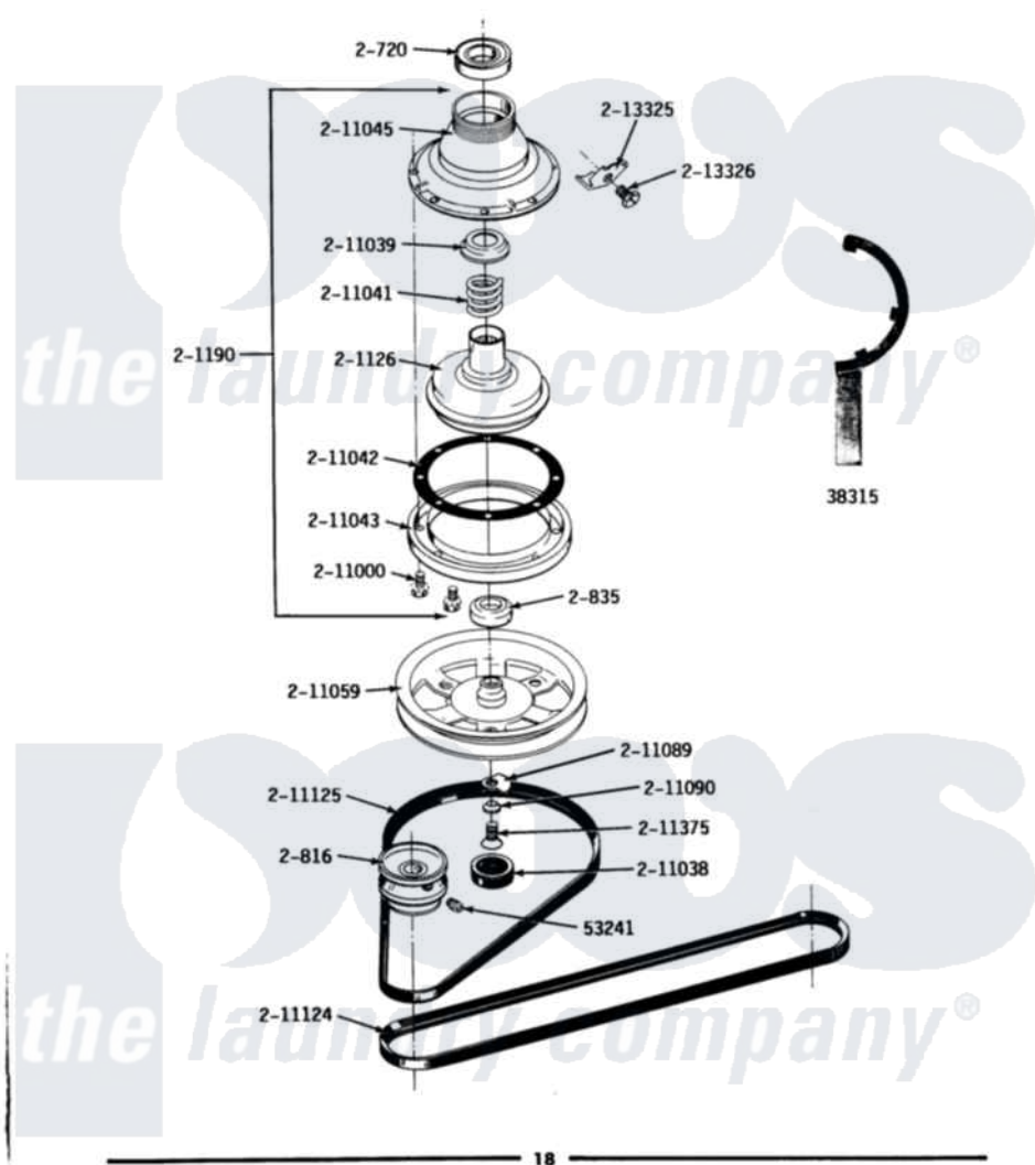
Maytag Commercial Maytag A23CDL Washer Parts Parts Diagram 09 - CLUTCH\BRAKE\BELTS Click on the part number to view part
