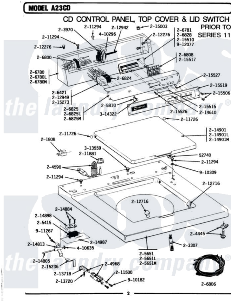
Maytag Commercial Maytag A23CDW Washer Parts Parts Diagram 01 - CD CONTROL PANEL, TOP COVER & LID SWITCH
