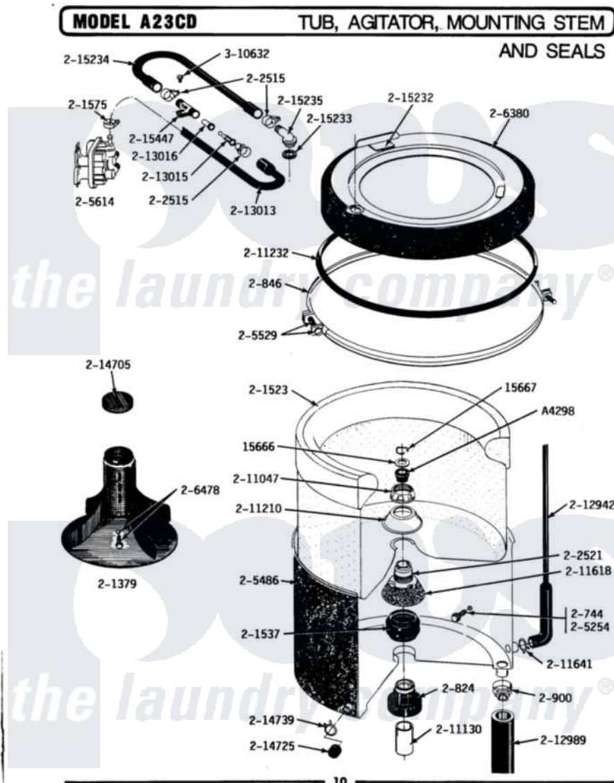
Maytag Commercial Maytag A23CDW Washer Parts Parts Diagram 05 - TUB/AGITATOR Click on the part number to view part
