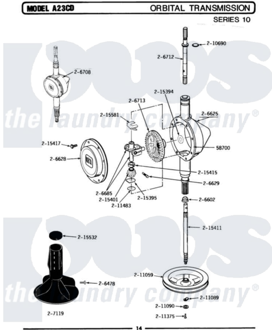
Maytag Commercial Maytag A23CDW Washer Parts Parts Diagram 07 - ORBITAL TRANSMISSION Click on the part number to view part
