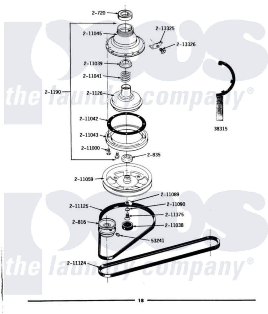
Maytag Commercial Maytag A23CDW Washer Parts Parts Diagram 09 - CLUTCH\BRAKE\BELTS Click on the part number to view part
