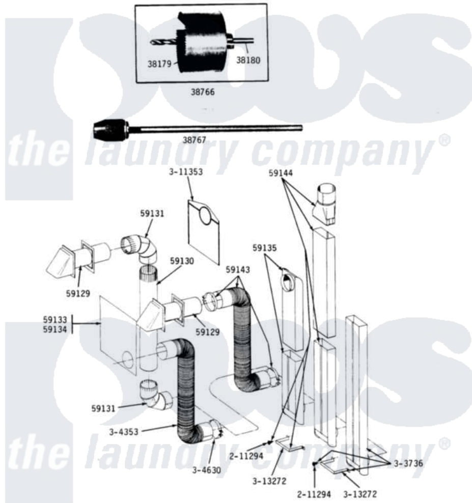
Maytag Commercial Maytag DG16CM Dryer Parts Parts Diagram 11 - INSTALLATION ACCESSORIES Click on the part number to view part
