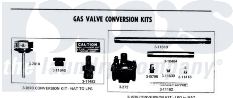
Maytag Commercial Maytag DG16CT Dryer Parts Parts Diagram 10 - GAS VALVE (ORIGINAL) Click on the part number to view part
