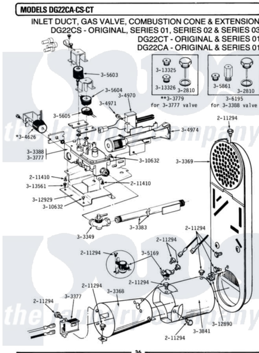
Maytag Commercial Maytag DG22CT Dryer Parts Parts Diagram 09 - INLET DUCT, GAS VALVE & COMBUSTION CONE
