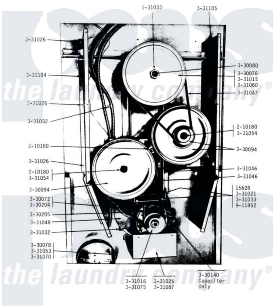
Maytag Commercial Maytag DG30CMD Dryer Parts Parts Diagram 09 - REAR VIEW-SHIELD REMOVED Click on the part number to view part
