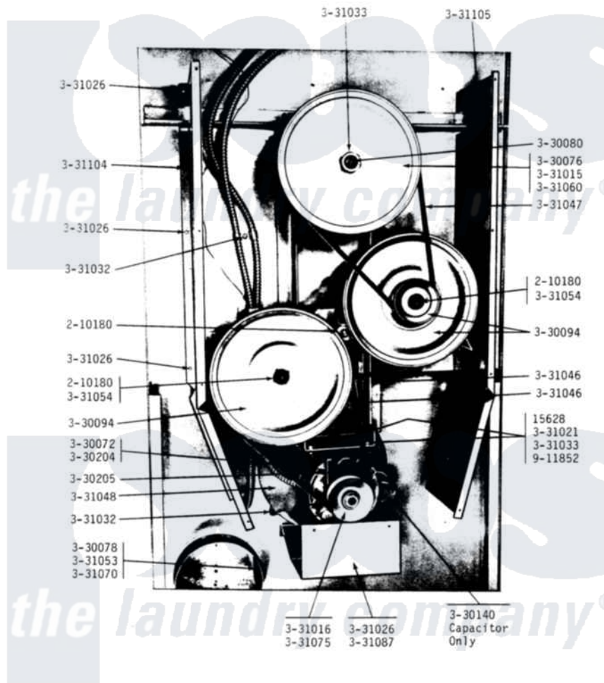
Maytag Commercial Maytag DG30CT Dryer Parts Parts Diagram 12 - REAR VIEW-SHIELD REMOVED Click on the part number to view part
