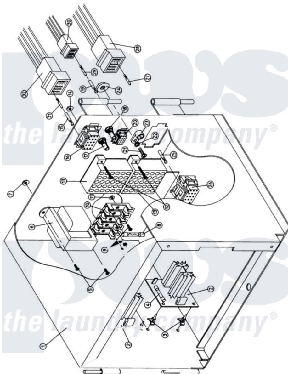
Maytag Commercial Maytag DGS30PC1 Dryer Parts Parts Diagram 04 - DUAL CTRL MICROPROCESSOR (DMC) CNTRL BOX
