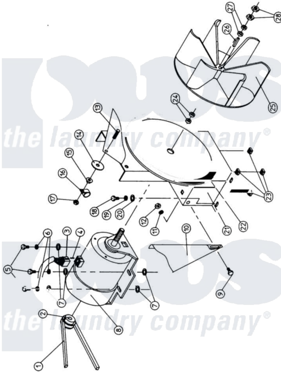
Maytag Commercial Maytag DGS30PC1 Dryer Parts Parts Diagram 14 - FAN-COOLED MOTOR MOUNT ASSEMBLY Click on the part number to view part
