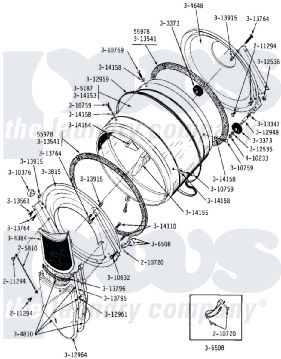
Maytag Commercial Maytag GDE23CD Dryer Parts Parts Diagram 05 - LINT SCREEN, TUMBLER (FRONT & BACK)
